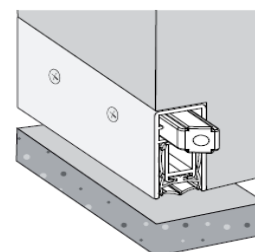
DRS 1530 SEMI RECESSED
