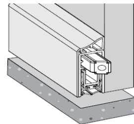
DRS 1530 FACE MOUNTED
